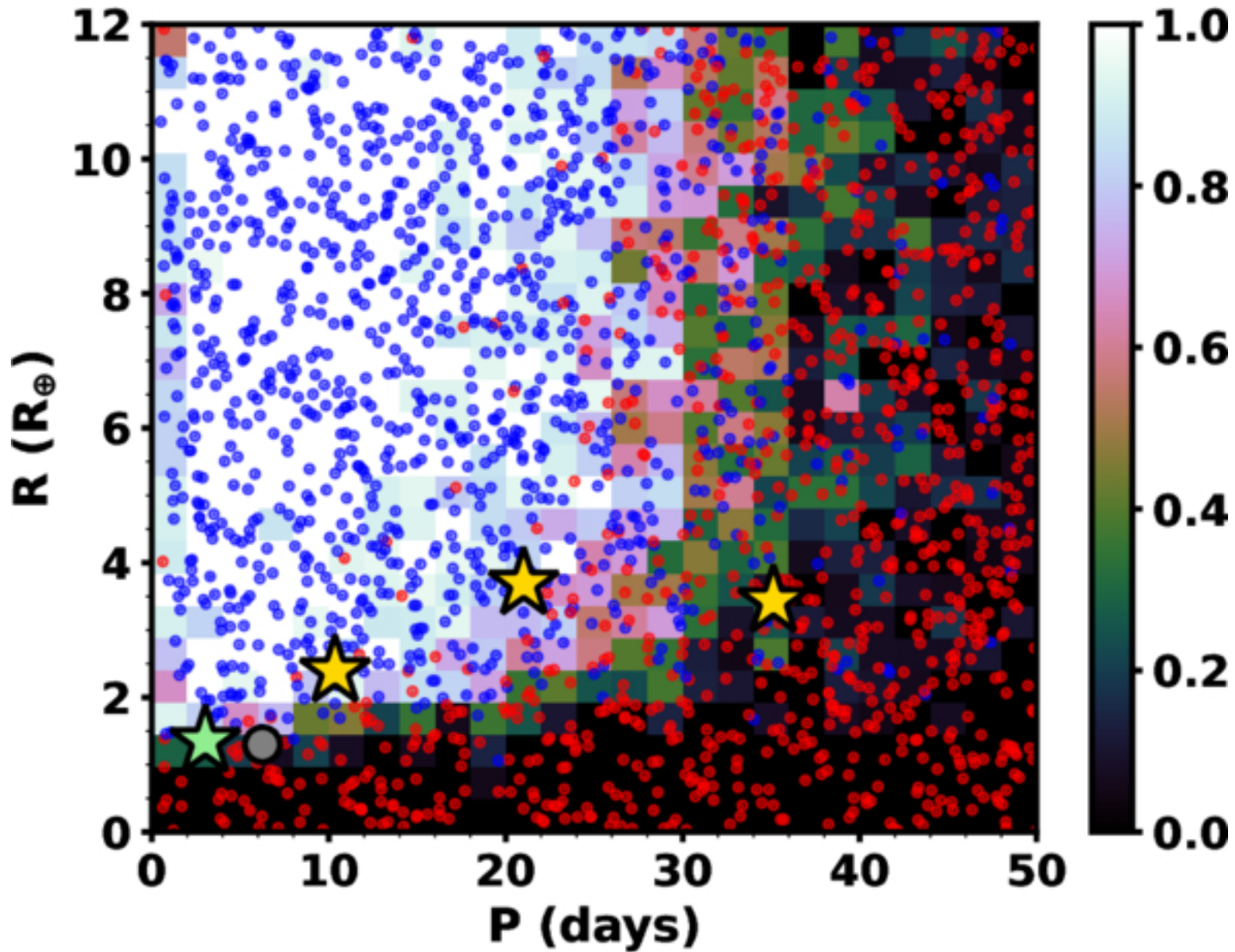
Figure 3. from Madyson G. Barber et al 2025 Astron. J. 170 doi:10.3847/1538-3881/add7db https://dx.doi.org/10.3847/1538-3881/add7db © 2025. The Author(s). Published by the American Astronomical Society.
