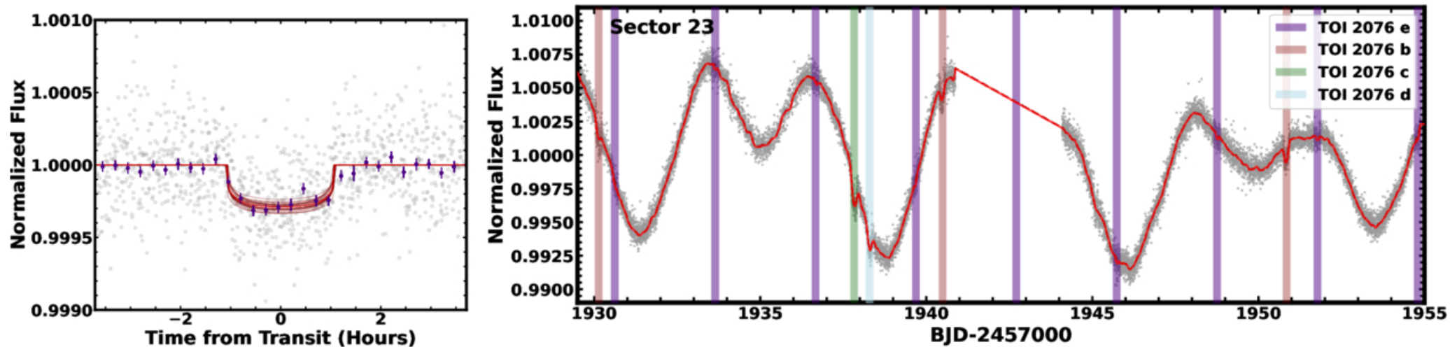
Figure 2. from Madyson G. Barber et al 2025 Astron. J. 170 doi:10.3847/1538-3881/add7db https://dx.doi.org/10.3847/1538-3881/add7db © 2025. The Author(s). Published by the American Astronomical Society.
