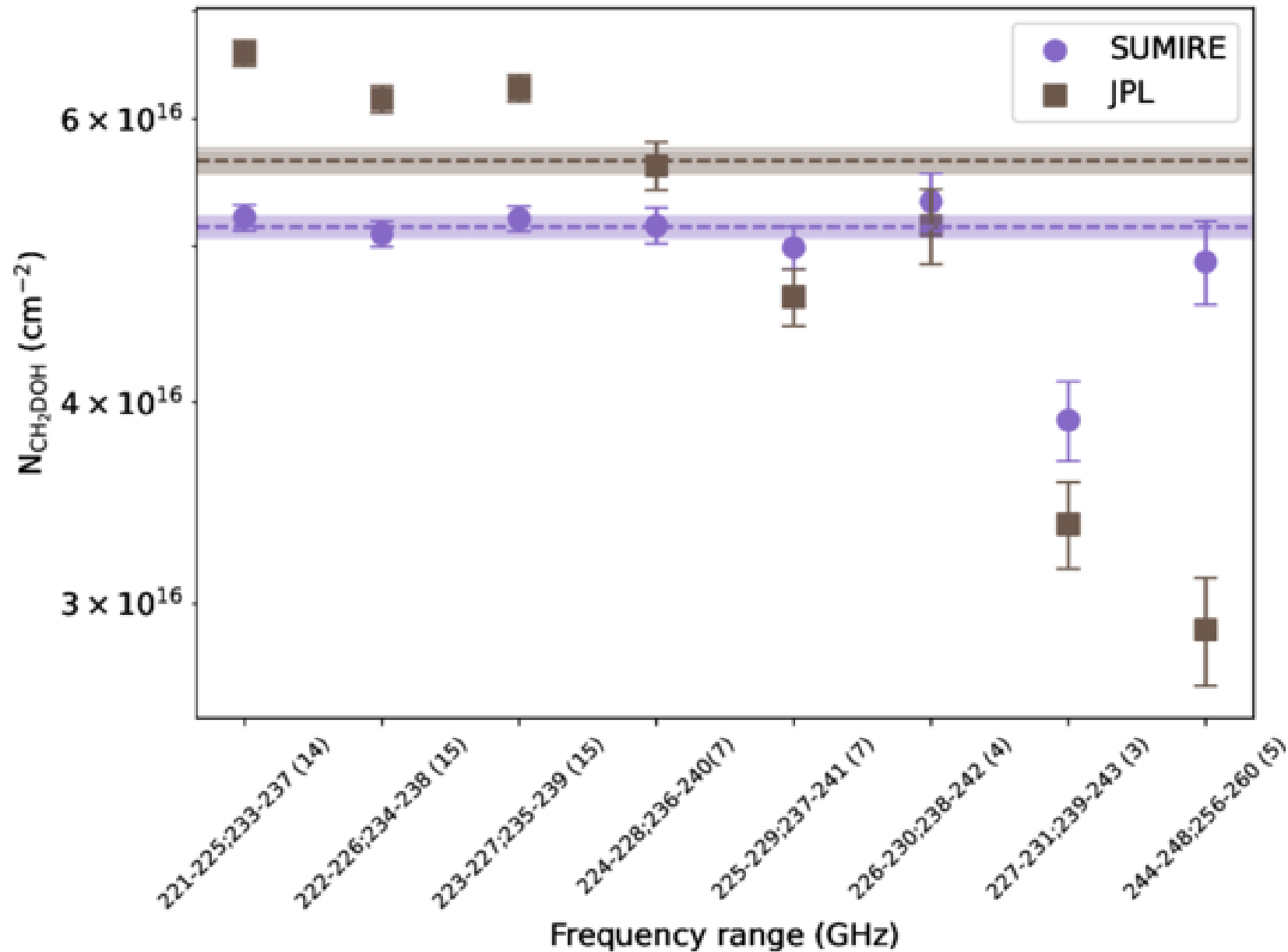
Figure 3. from Shaoshan Zeng et al 2025 Astron. J. 170 doi:10.3847/1538-3881/add733 https://dx.doi.org/10.3847/1538-3881/add733 © 2025. The Author(s). Published by the American Astronomical Society.
