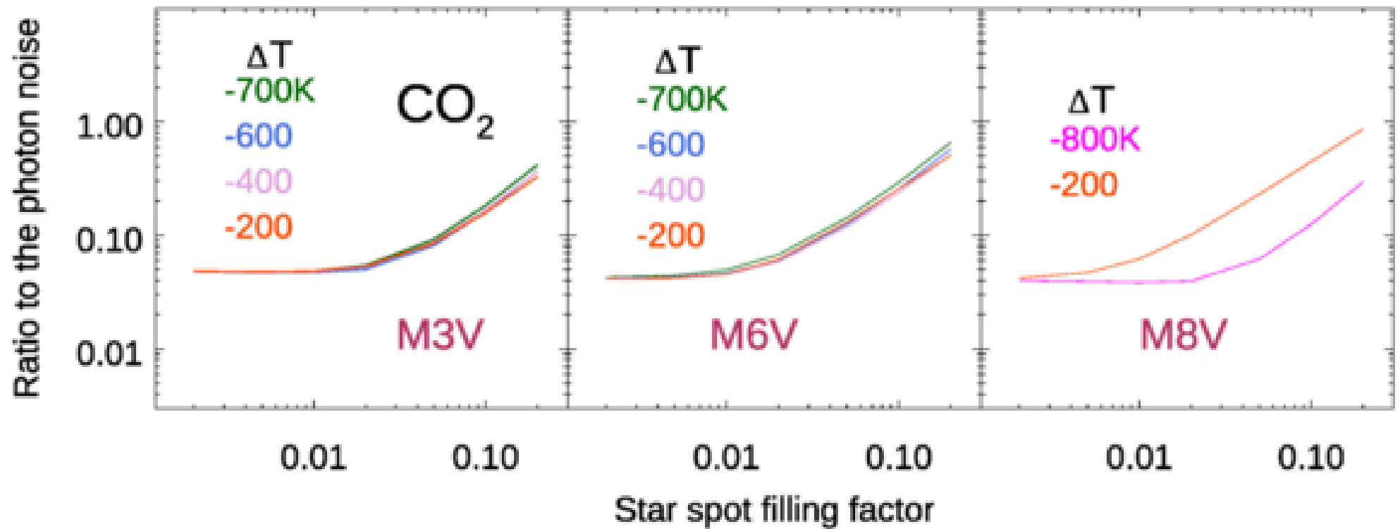
Figure 8. from Drake Deming et al 2025 Astron. J. 170 doi:10.3847/1538-3881/add531 https://dx.doi.org/10.3847/1538-3881/add531 © 2025. The Author(s). Published by the American Astronomical Society.
