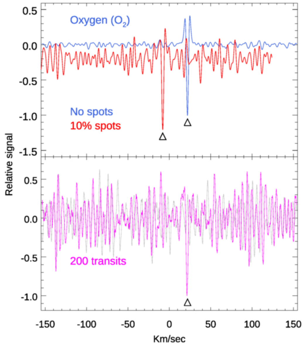
Figure 7. from Drake Deming et al 2025 Astron. J. 170 doi:10.3847/1538-3881/add531 https://dx.doi.org/10.3847/1538-3881/add531 © 2025. The Author(s). Published by the American Astronomical Society.
