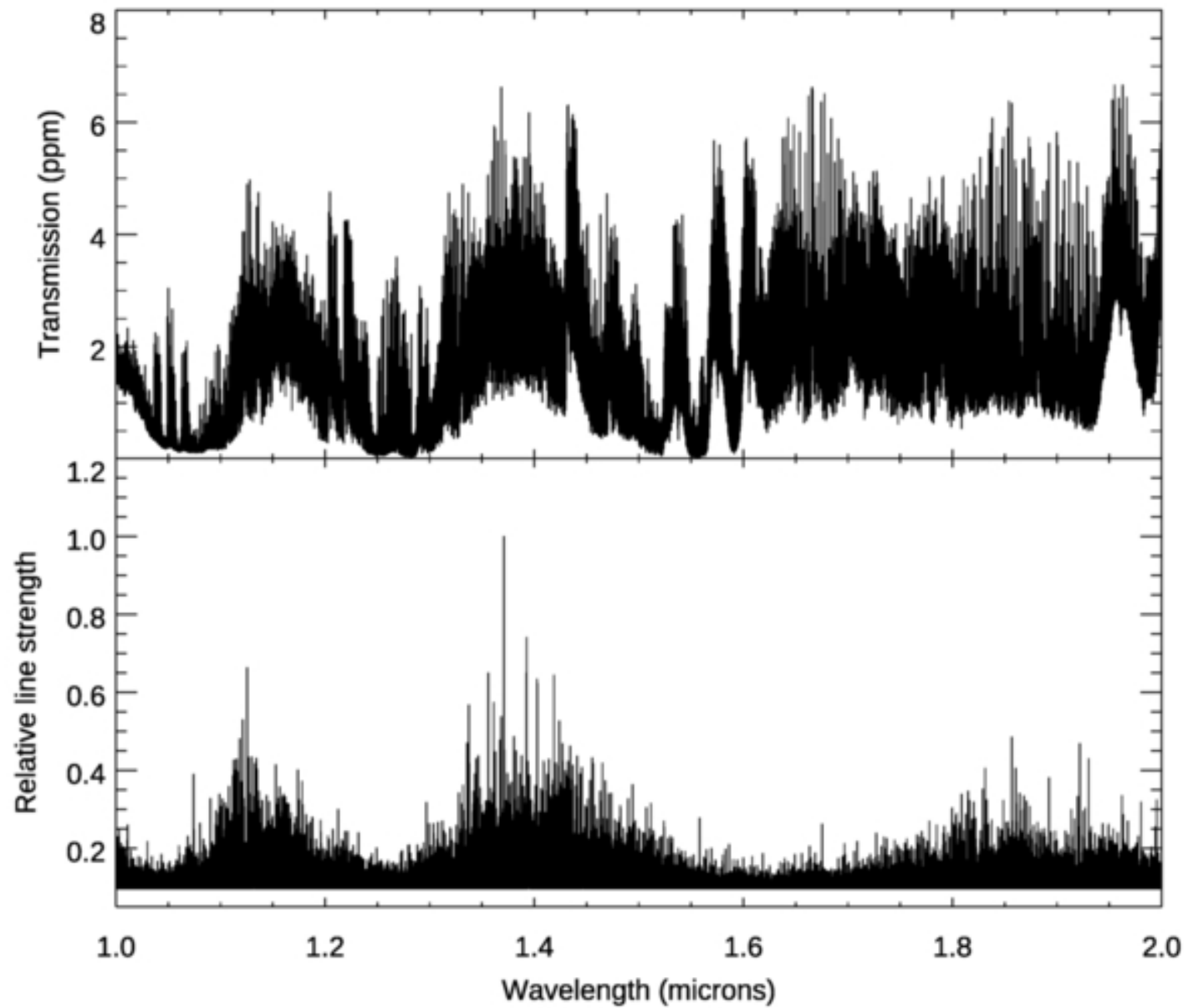
Figure 2. from Drake Deming et al 2025 Astron. J. 170 doi:10.3847/1538-3881/add531 https://dx.doi.org/10.3847/1538-3881/add531 © 2025. The Author(s). Published by the American Astronomical Society.
