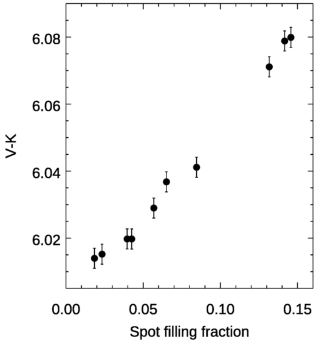
Figure 13. from Drake Deming et al 2025 Astron. J. 170 doi:10.3847/1538-3881/add531 https://dx.doi.org/10.3847/1538-3881/add531 © 2025. The Author(s). Published by the American Astronomical Society.
