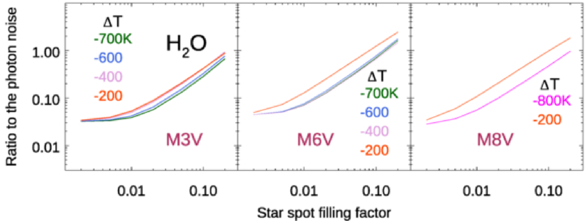
Figure 11. from Drake Deming et al 2025 Astron. J. 170 doi:10.3847/1538-3881/add531 https://dx.doi.org/10.3847/1538-3881/add531 © 2025. The Author(s). Published by the American Astronomical Society.
