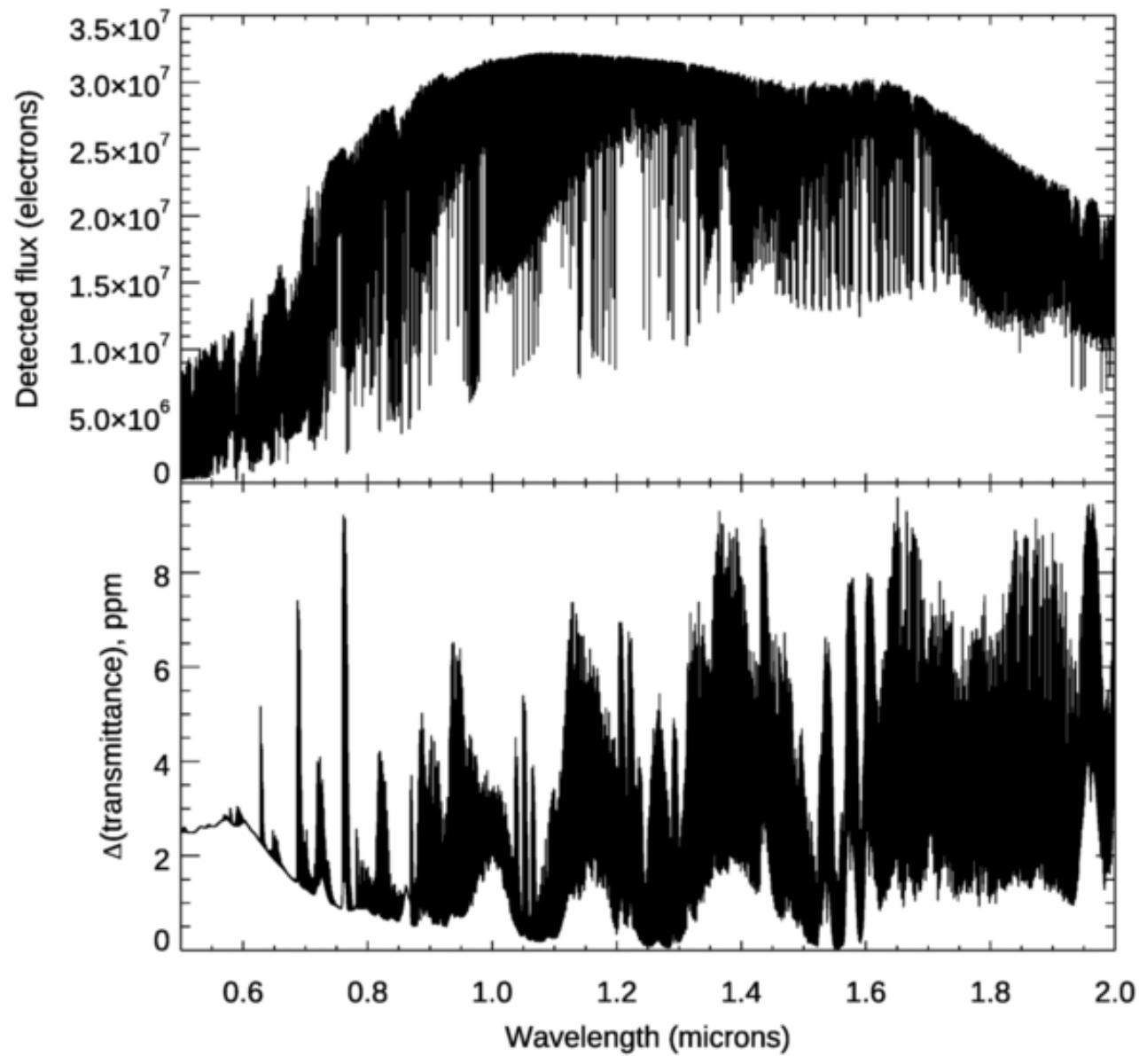
Figure 1. from Drake Deming et al 2025 Astron. J. 170 doi:10.3847/1538-3881/add531 https://dx.doi.org/10.3847/1538-3881/add531 © 2025. The Author(s). Published by the American Astronomical Society.
