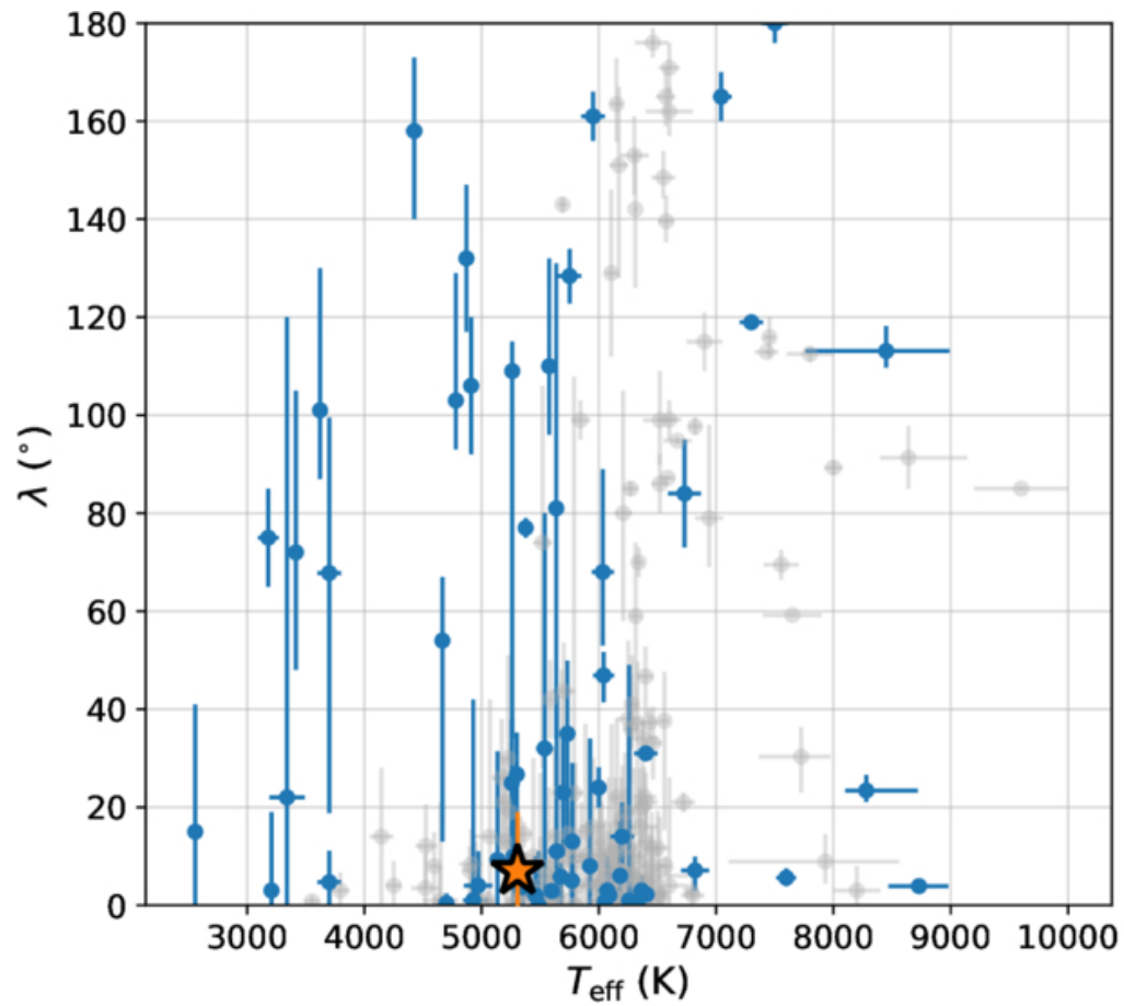
Figure 4. from Patrick Tamburo et al 2025 Astron. J. 170 doi:10.3847/1538-3881/add530 https://dx.doi.org/10.3847/1538-3881/add530 © 2025. The Author(s). Published by the American Astronomical Society.
