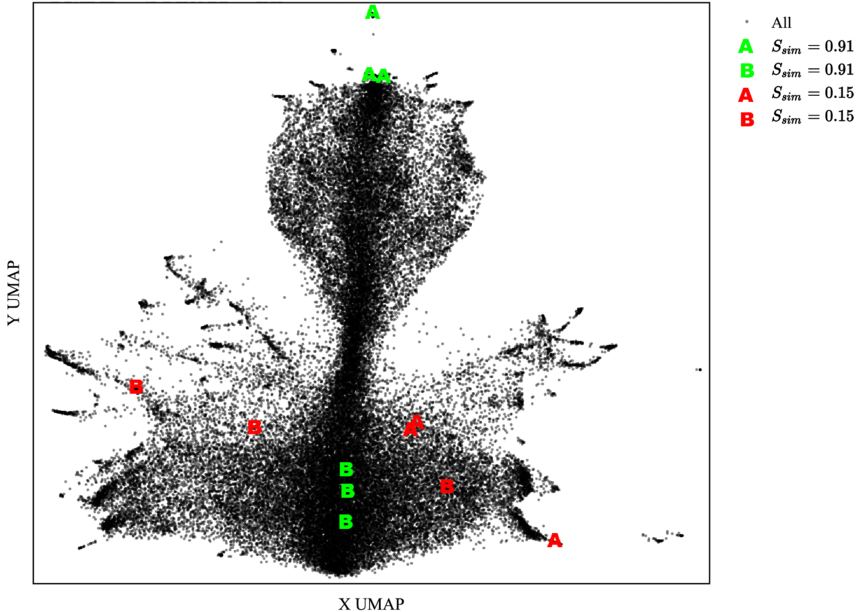
Figure 7. from Snir Pardo et al 2025 Astron. J. 170 doi:10.3847/1538-3881/add52b https://dx.doi.org/10.3847/1538-3881/add52b © 2025. The Author(s). Published by the American Astronomical Society.
