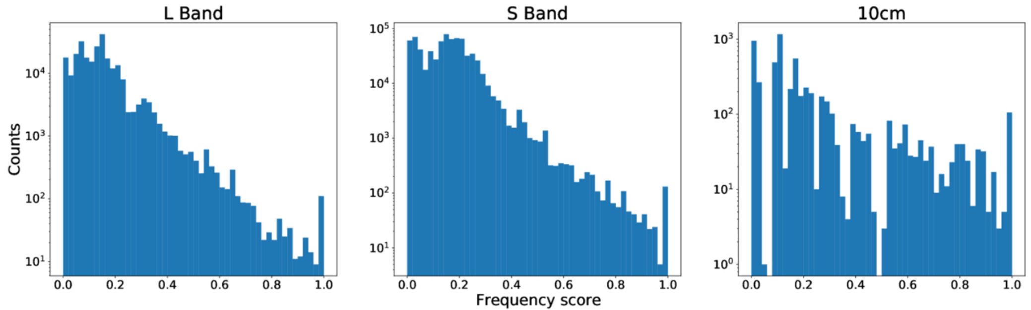
Figure 6. from Snir Pardo et al 2025 Astron. J. 170 doi:10.3847/1538-3881/add52b https://dx.doi.org/10.3847/1538-3881/add52b © 2025. The Author(s). Published by the American Astronomical Society.
