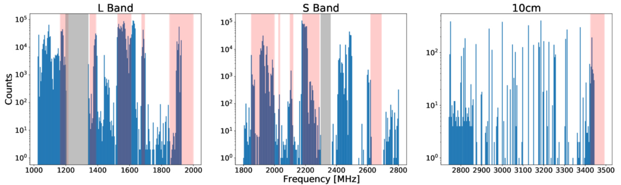
Figure 5. from Snir Pardo et al 2025 Astron. J. 170 doi:10.3847/1538-3881/add52b https://dx.doi.org/10.3847/1538-3881/add52b © 2025. The Author(s). Published by the American Astronomical Society.
