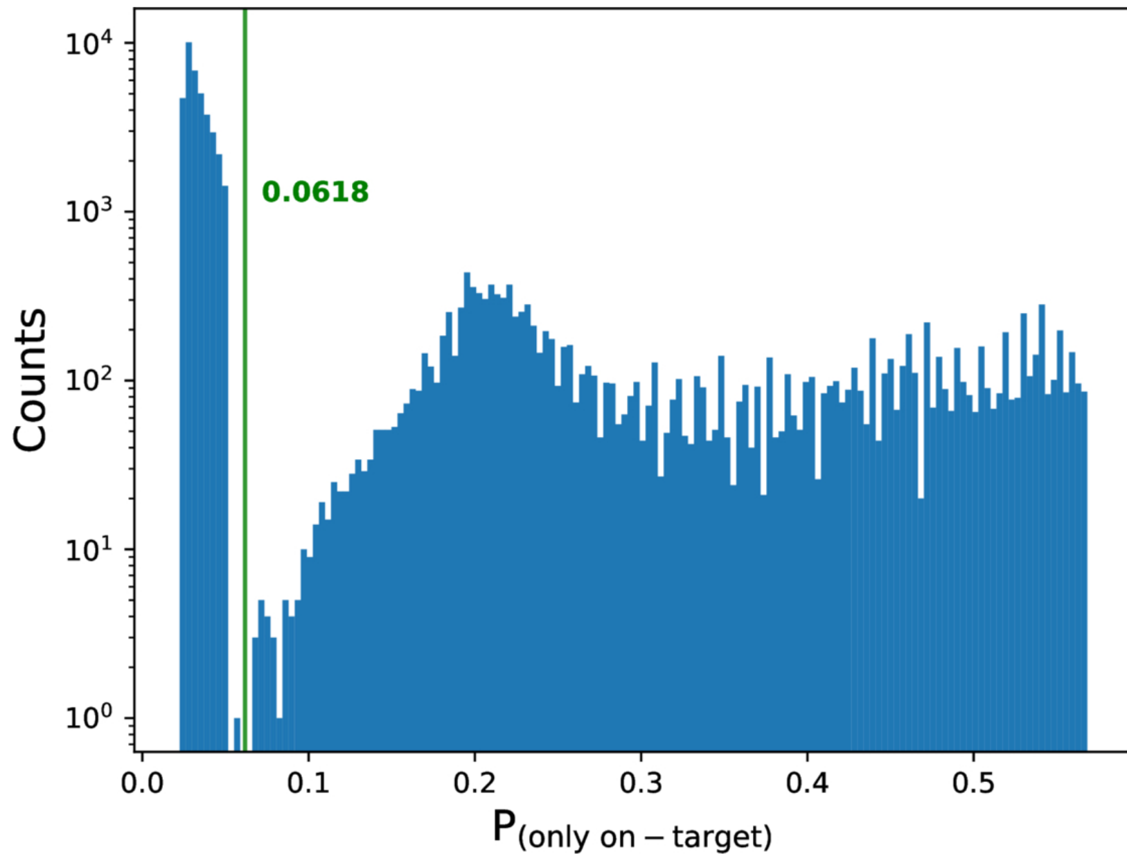
Figure 4. from Snir Pardo et al 2025 Astron. J. 170 doi:10.3847/1538-3881/add52b https://dx.doi.org/10.3847/1538-3881/add52b © 2025. The Author(s). Published by the American Astronomical Society.
