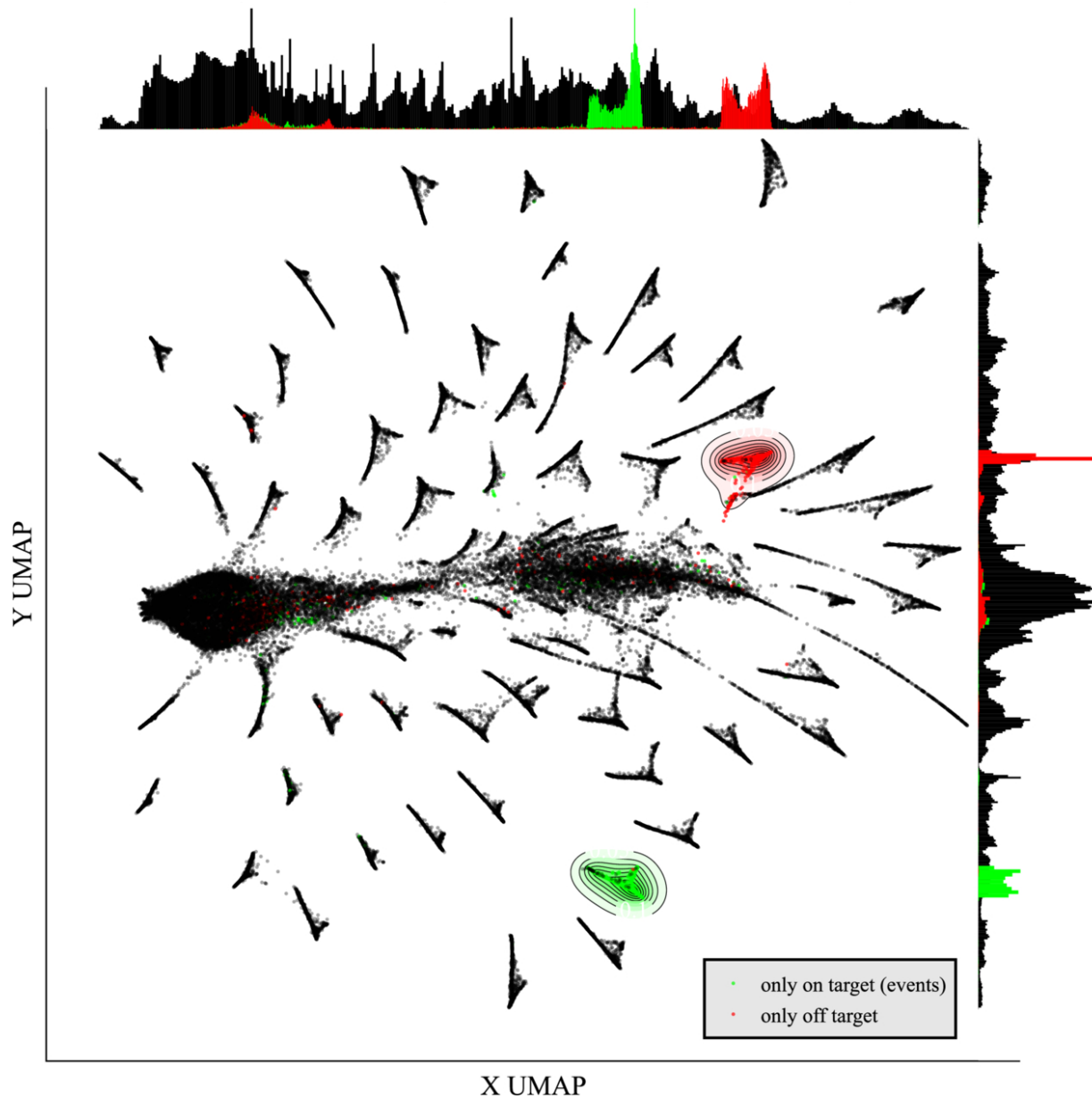
Figure 3. from Snir Pardo et al 2025 Astron. J. 170 doi:10.3847/1538-3881/add52b https://dx.doi.org/10.3847/1538-3881/add52b © 2025. The Author(s). Published by the American Astronomical Society.
