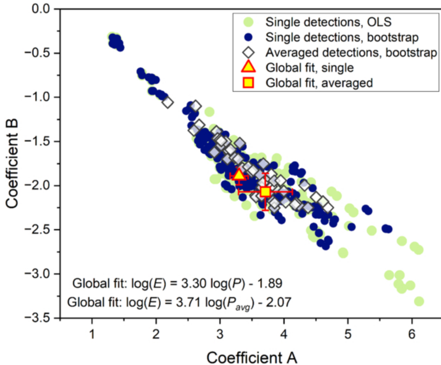
Figure 9. from Elizabeth A. Silber et al 2025 Astron. J. 170 doi:10.3847/1538-3881/add47d https://dx.doi.org/10.3847/1538-3881/add47d © 2025. The Author(s). Published by the American Astronomical Society.
