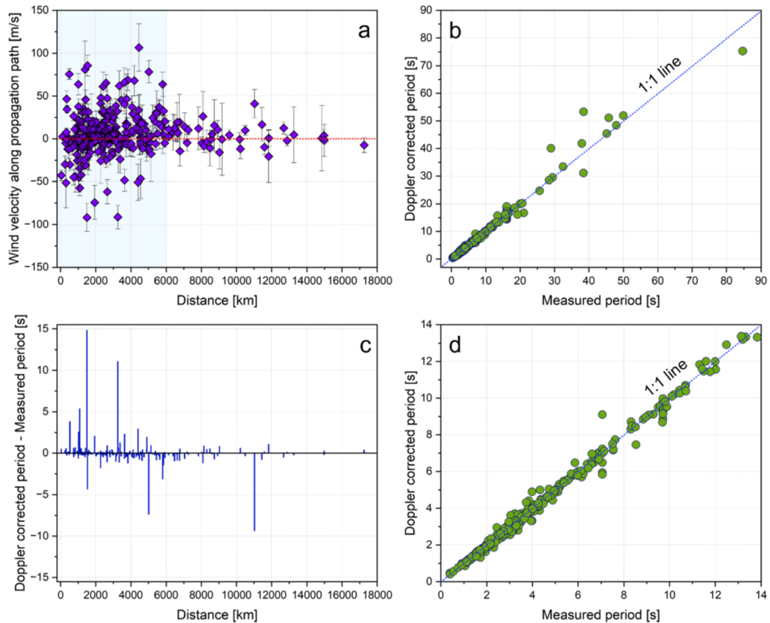
Figure 8. from Elizabeth A. Silber et al 2025 Astron. J. 170 doi:10.3847/1538-3881/add47d https://dx.doi.org/10.3847/1538-3881/add47d © 2025. The Author(s). Published by the American Astronomical Society.
