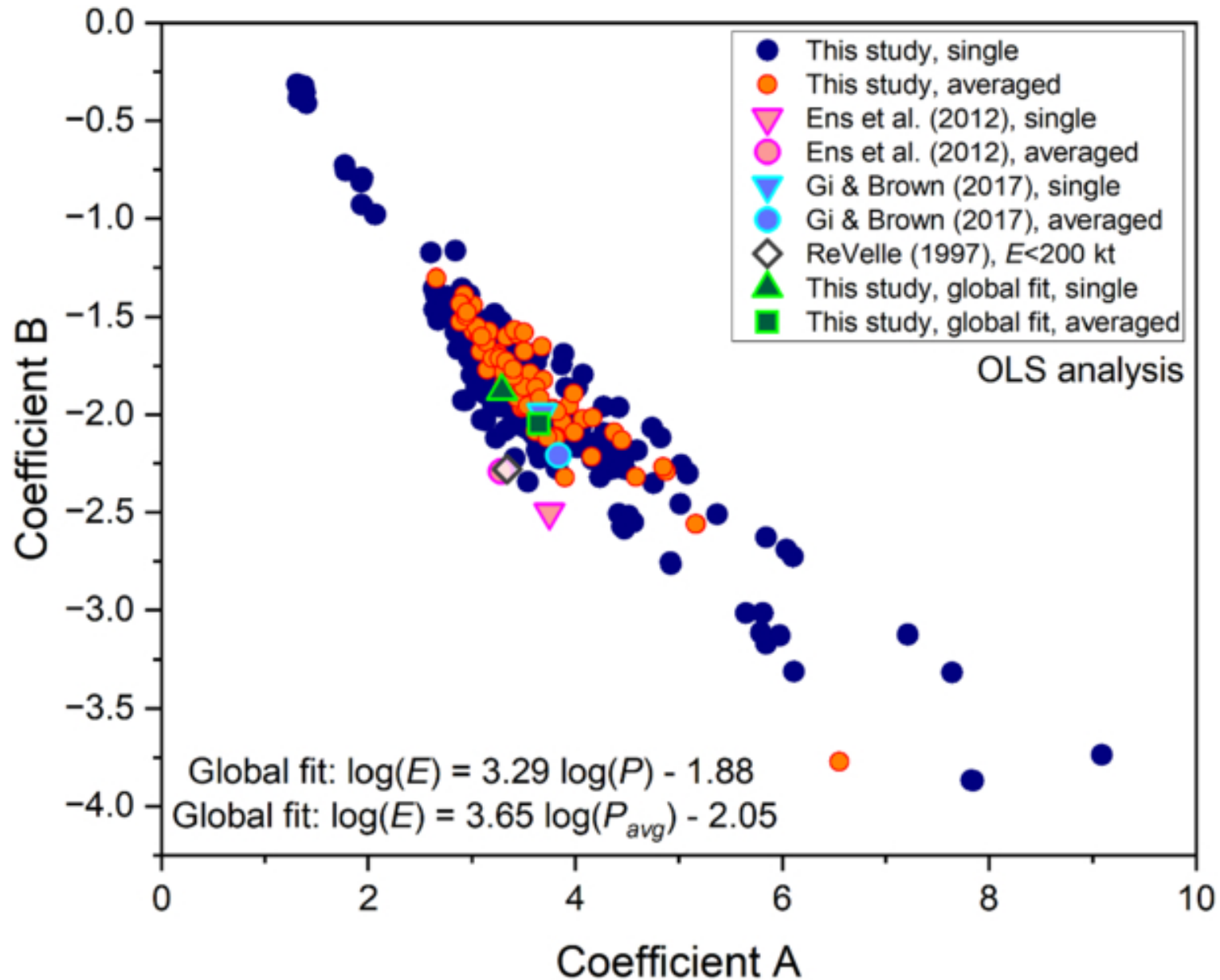
Figure 6. from Elizabeth A. Silber et al 2025 Astron. J. 170 doi:10.3847/1538-3881/add47d https://dx.doi.org/10.3847/1538-3881/add47d © 2025. The Author(s). Published by the American Astronomical Society.
