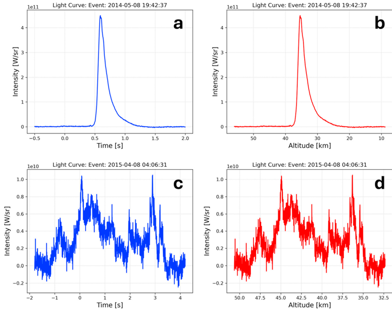
Figure 5. from Elizabeth A. Silber et al 2025 Astron. J. 170 doi:10.3847/1538-3881/add47d https://dx.doi.org/10.3847/1538-3881/add47d © 2025. The Author(s). Published by the American Astronomical Society.
