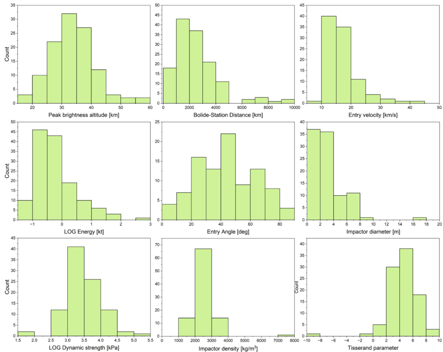
Figure 4. from Elizabeth A. Silber et al 2025 Astron. J. 170 doi:10.3847/1538-3881/add47d https://dx.doi.org/10.3847/1538-3881/add47d © 2025. The Author(s). Published by the American Astronomical Society.
