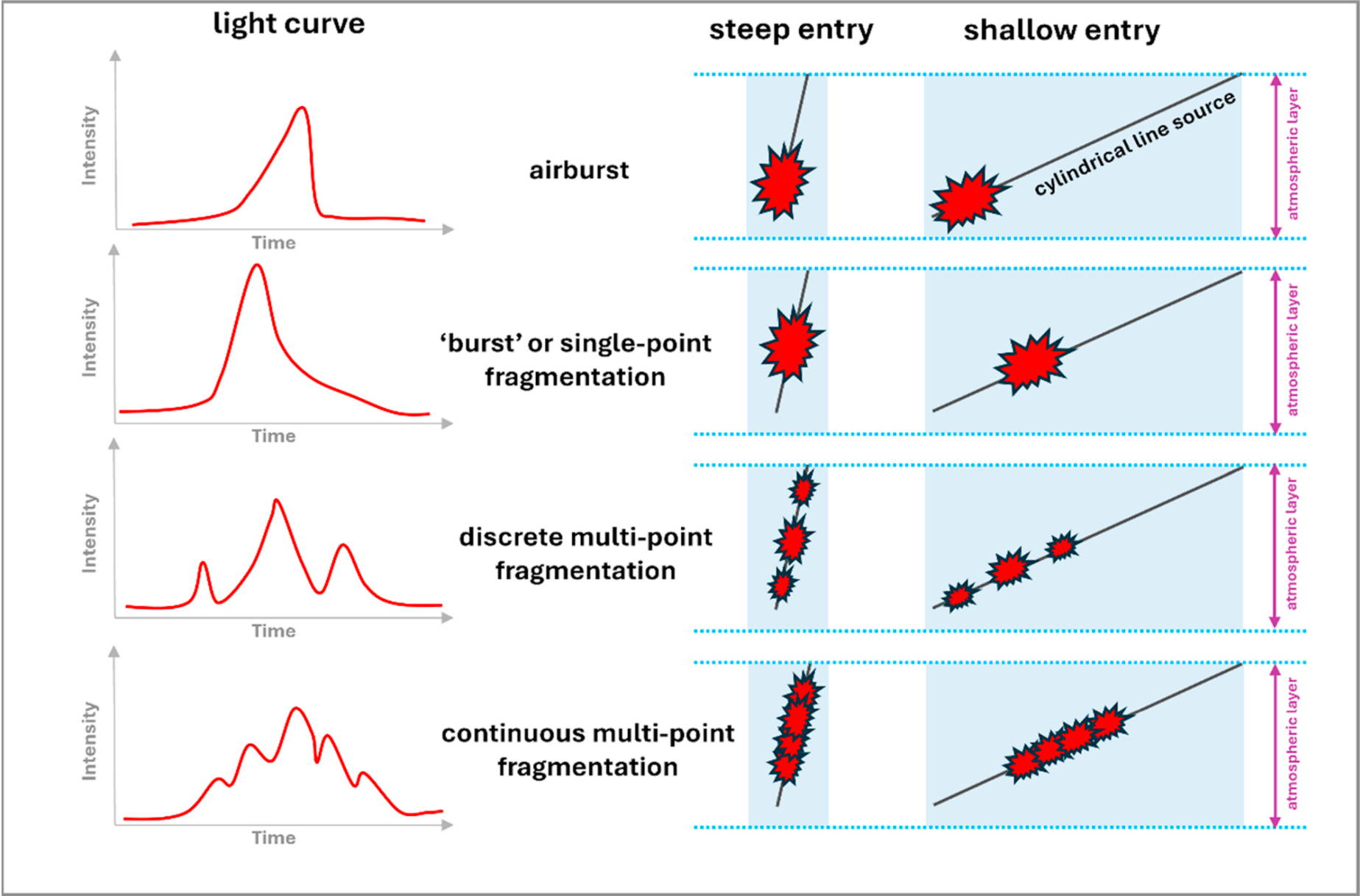
Figure 2. from Elizabeth A. Silber et al 2025 Astron. J. 170 doi:10.3847/1538-3881/add47d https://dx.doi.org/10.3847/1538-3881/add47d © 2025. The Author(s). Published by the American Astronomical Society.
