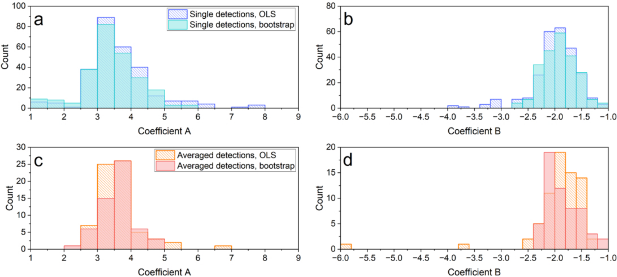
Figure 10. from Elizabeth A. Silber et al 2025 Astron. J. 170 doi:10.3847/1538-3881/add47d https://dx.doi.org/10.3847/1538-3881/add47d © 2025. The Author(s). Published by the American Astronomical Society.
