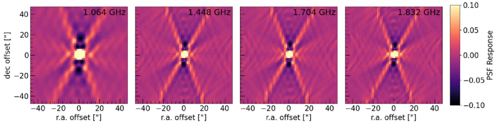
Figure 9. from Nicholas M. Luber et al 2025 Astron. J. 170 doi:10.3847/1538-3881/add2f2 https://dx.doi.org/10.3847/1538-3881/add2f2 © 2025. The Author(s). Published by the American Astronomical Society.
