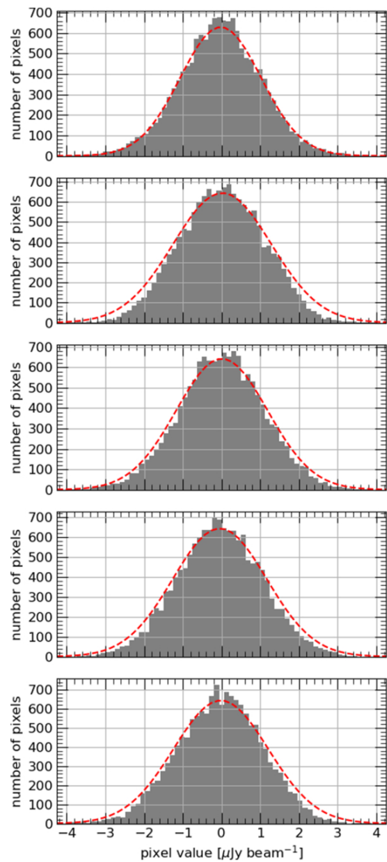
Figure 7. from Nicholas M. Lubet et al 2025 Astron. J. 170 doi:10.3847/1538-3881/add2f2 https://dx.doi.org/10.3847/1538-3881/add2f2 © 2025. The Author(s). Published by the American Astronomical Society.
