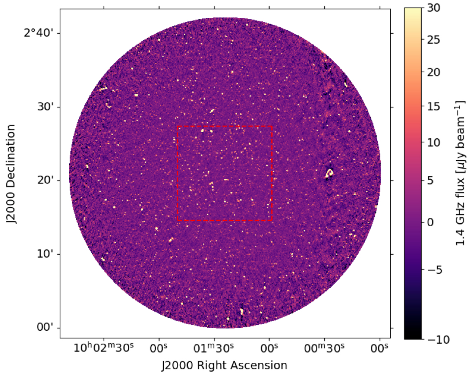
Figure 5. from Nicholas M. Luber et al 2025 Astron. J. 170 doi:10.3847/1538-3881/add2f2 https://dx.doi.org/10.3847/1538-3881/add2f2 © 2025. The Author(s). Published by the American Astronomical Society.
