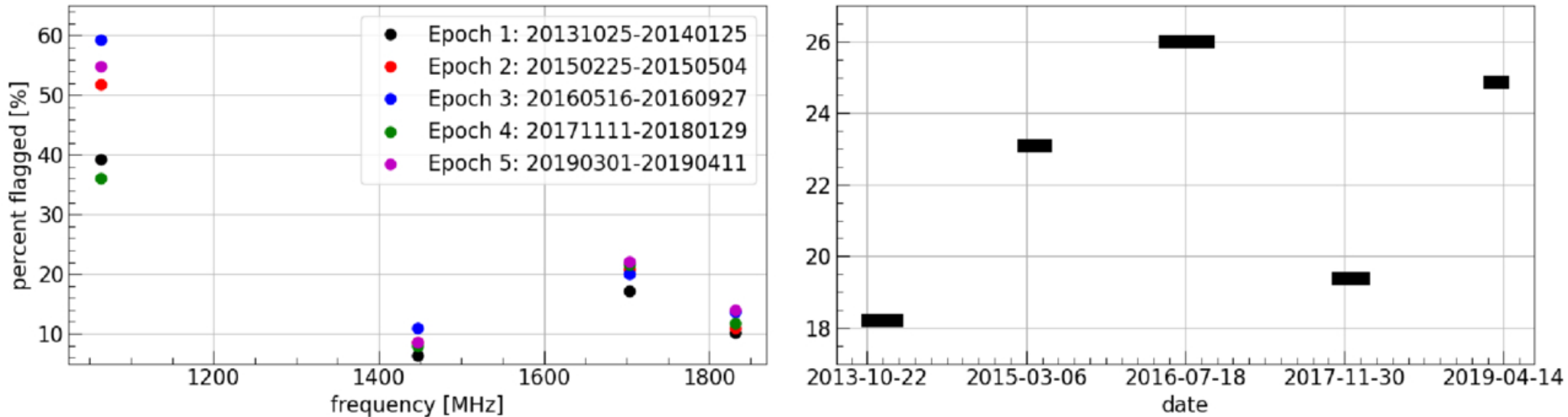
Figure 4. from Nicholas M. Luber et al 2025 Astron. J. 170 doi:10.3847/1538-3881/add2f2 https://dx.doi.org/10.3847/1538-3881/add2f2 © 2025. The Author(s). Published by the American Astronomical Society.
