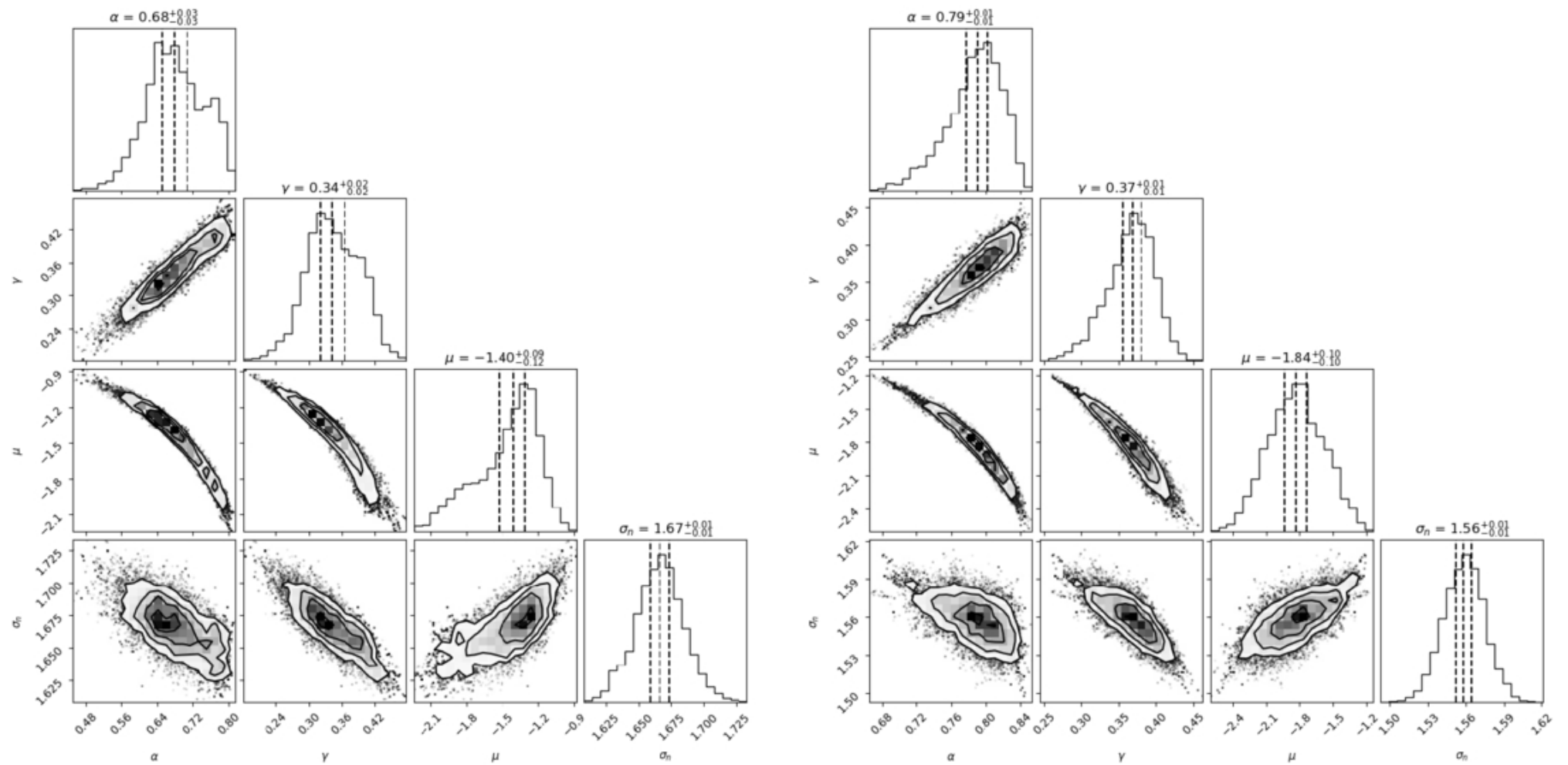
Figure 15. from Nicholas M. Lubner et al 2025 Astron. J. 170 doi:10.3847/1538-3881/add2f2 https://dx.doi.org/10.3847/1538-3881/add2f2 © 2025. The Author(s). Published by the American Astronomical Society.
