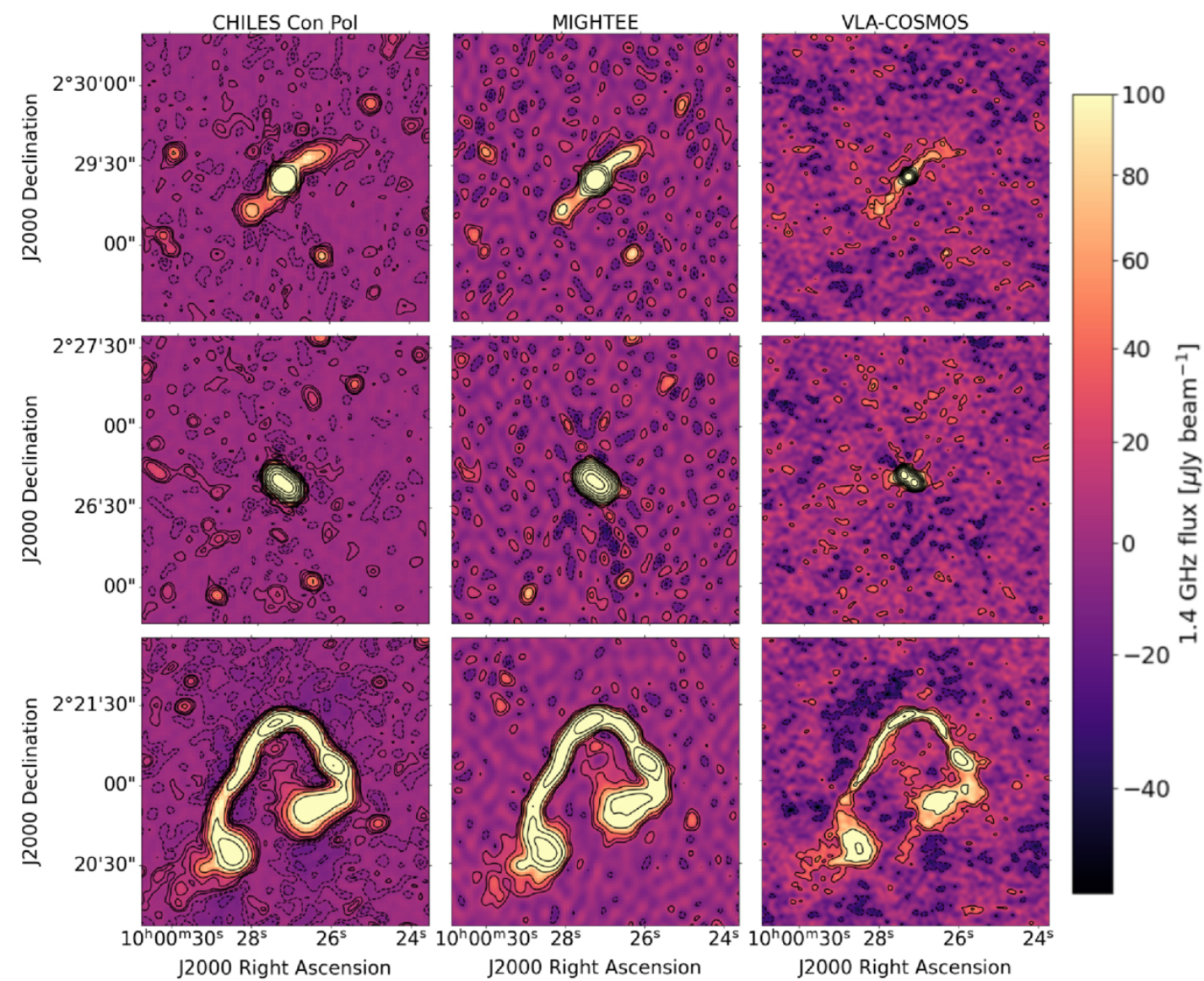
Figure 13. from Nicholas M. Luber et al 2025 Astron. J. 170 doi:10.3847/1538-3881/add2f2 https://dx.doi.org/10.3847/1538-3881/add2f2 © 2025. The Author(s). Published by the American Astronomical Society.
