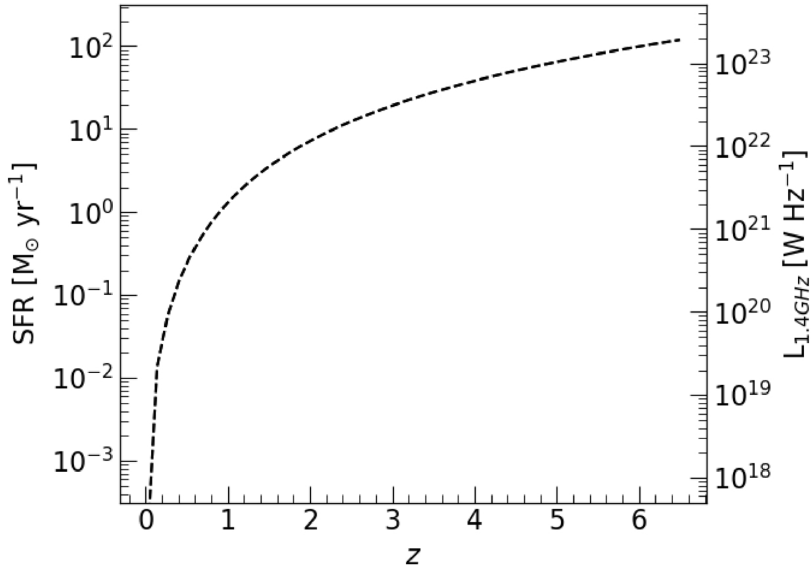
Figure 11. from Nicholas M. Luber et al 2025 Astron. J. 170 doi:10.3847/1538-3881/add2f2 https://dx.doi.org/10.3847/1538-3881/add2f2 © 2025. The Author(s). Published by the American Astronomical Society.
