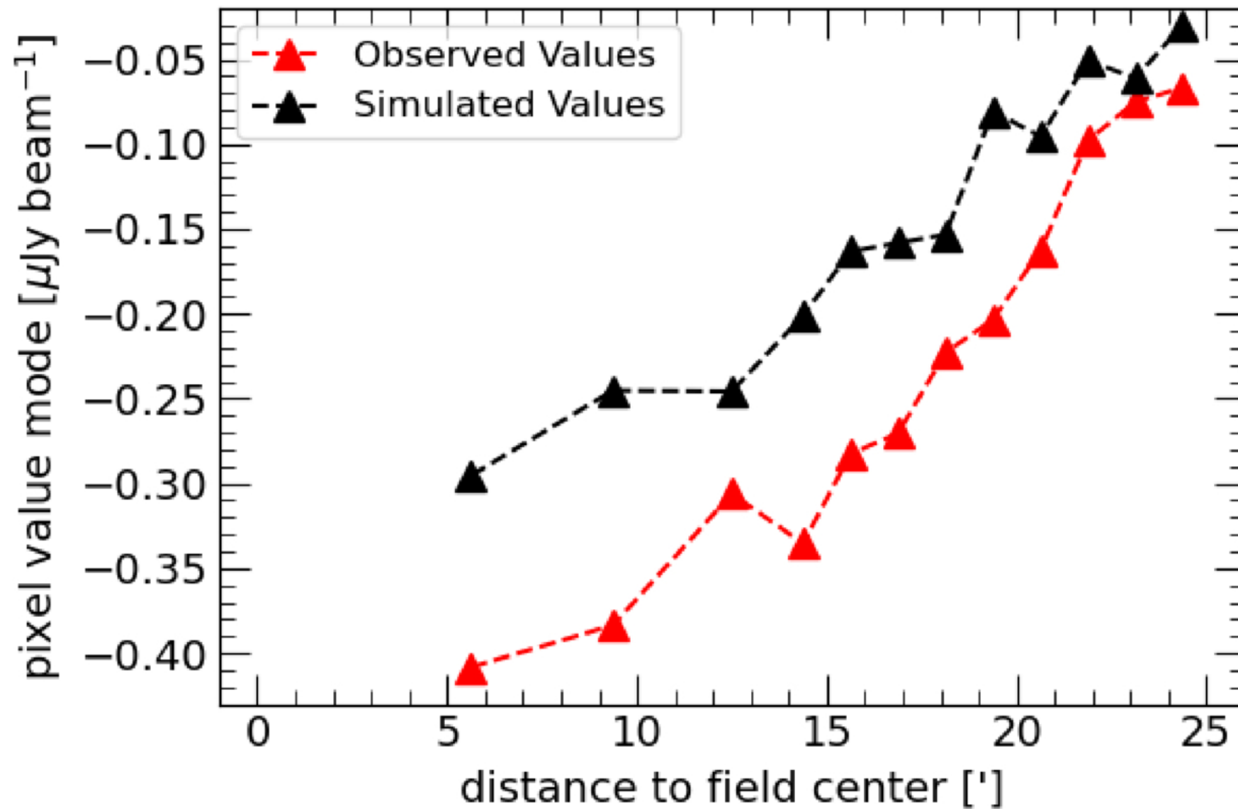
Figure 10. from Nicholas M. Luber et al 2025 Astron. J. 170 doi:10.3847/1538-3881/add2f2 https://dx.doi.org/10.3847/1538-3881/add2f2 © 2025. The Author(s). Published by the American Astronomical Society.
