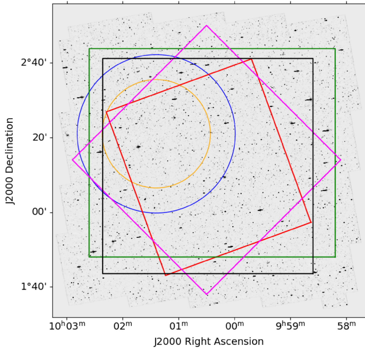
Figure 1. from Nicholas M. Luber et al 2025 Astron. J. 170 doi:10.3847/1538-3881/add2f2 https://dx.doi.org/10.3847/1538-3881/add2f2 © 2025. The Author(s). Published by the American Astronomical Society.
