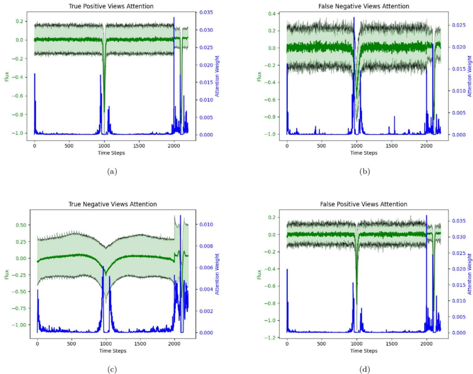
Figure 8. from Àlvar Hernández-Carnerero et al 2025 Astron. J. 170 doi:10.3847/1538-3881/add2f1 https://dx.doi.org/10.3847/1538-3881/add2f1 © 2025. The Author(s). Published by the American Astronomical Society.
