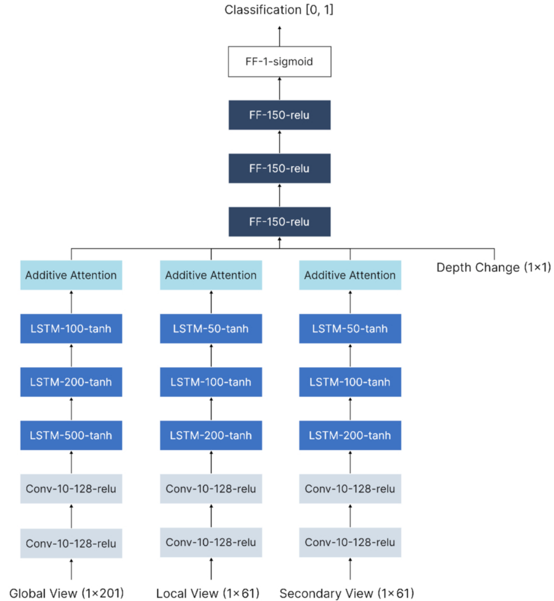
Figure 7. from Àlvar Hernández-Carnerero et al 2025 Astron. J. 170 doi:10.3847/1538-3881/add2f1 https://dx.doi.org/10.3847/1538-3881/add2f1 © 2025. The Author(s). Published by the American Astronomical Society.
