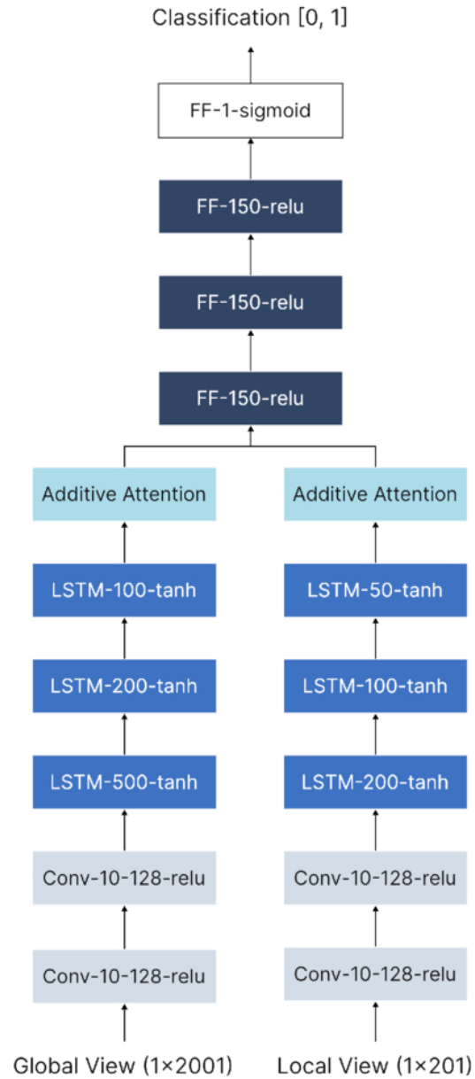
Figure 6. from Àlvar Hernández-Carnerero et al 2025 Astron. J. 170 doi:10.3847/1538-3881/add2f1 https://dx.doi.org/10.3847/1538-3881/add2f1 © 2025. The Author(s). Published by the American Astronomical Society.
