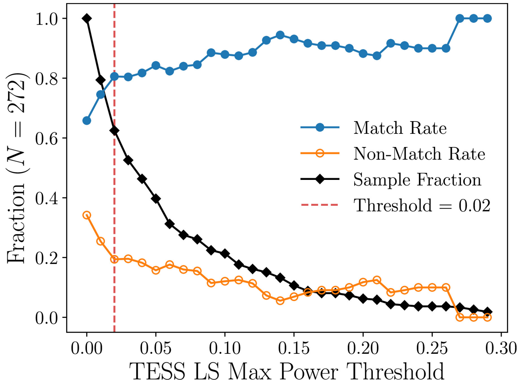
Figure 9. from Soichiro Hattori et al 2025 Astron. J. 170 doi:10.3847/1538-3881/add0ab https://dx.doi.org/10.3847/1538-3881/add0ab © 2025. The Author(s). Published by the American Astronomical Society.
