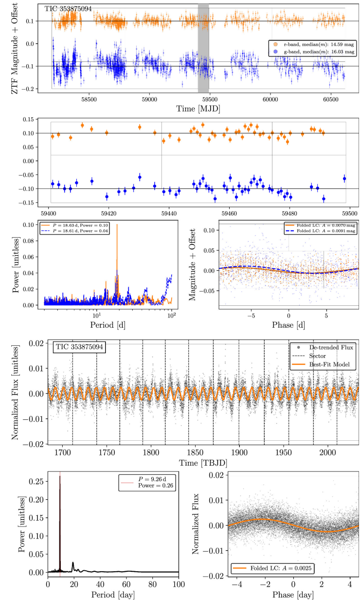
Figure 8. from Soichiro Hattori et al 2025 Astron. J. 170 doi:10.3847/1538-3881/add0ab https://dx.doi.org/10.3847/1538-3881/add0ab © 2025. The Author(s). Published by the American Astronomical Society.
