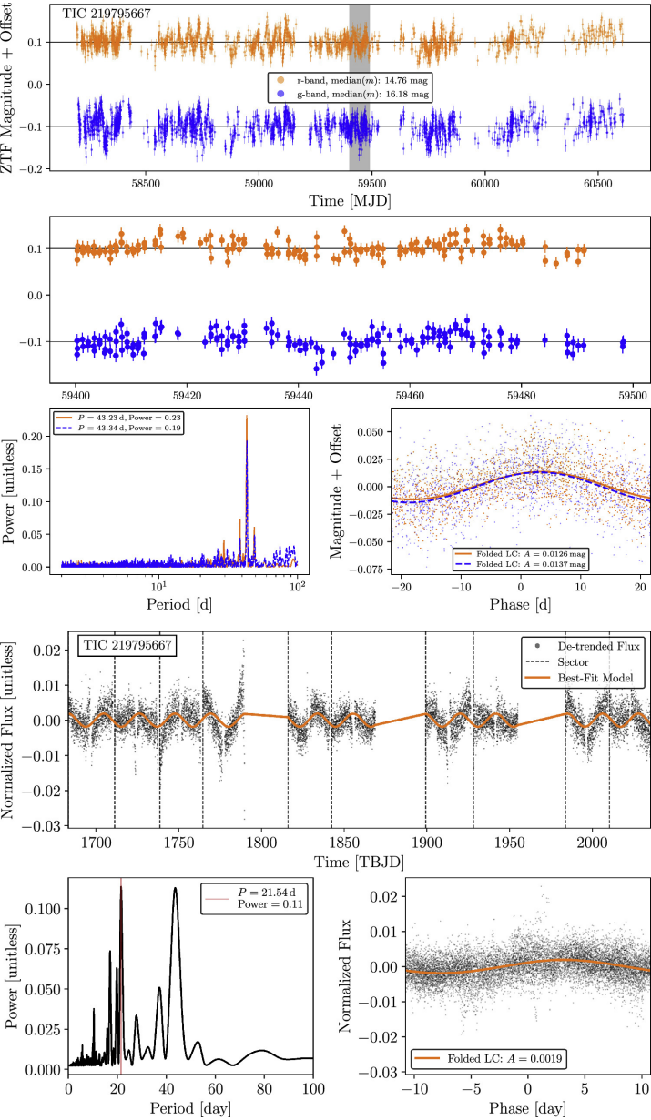
Figure 7. from Soichiro Hattori et al 2025 Astron. J. 170 doi:10.3847/1538-3881/add0ab https://dx.doi.org/10.3847/1538-3881/add0ab © 2025. The Author(s). Published by the American Astronomical Society.
