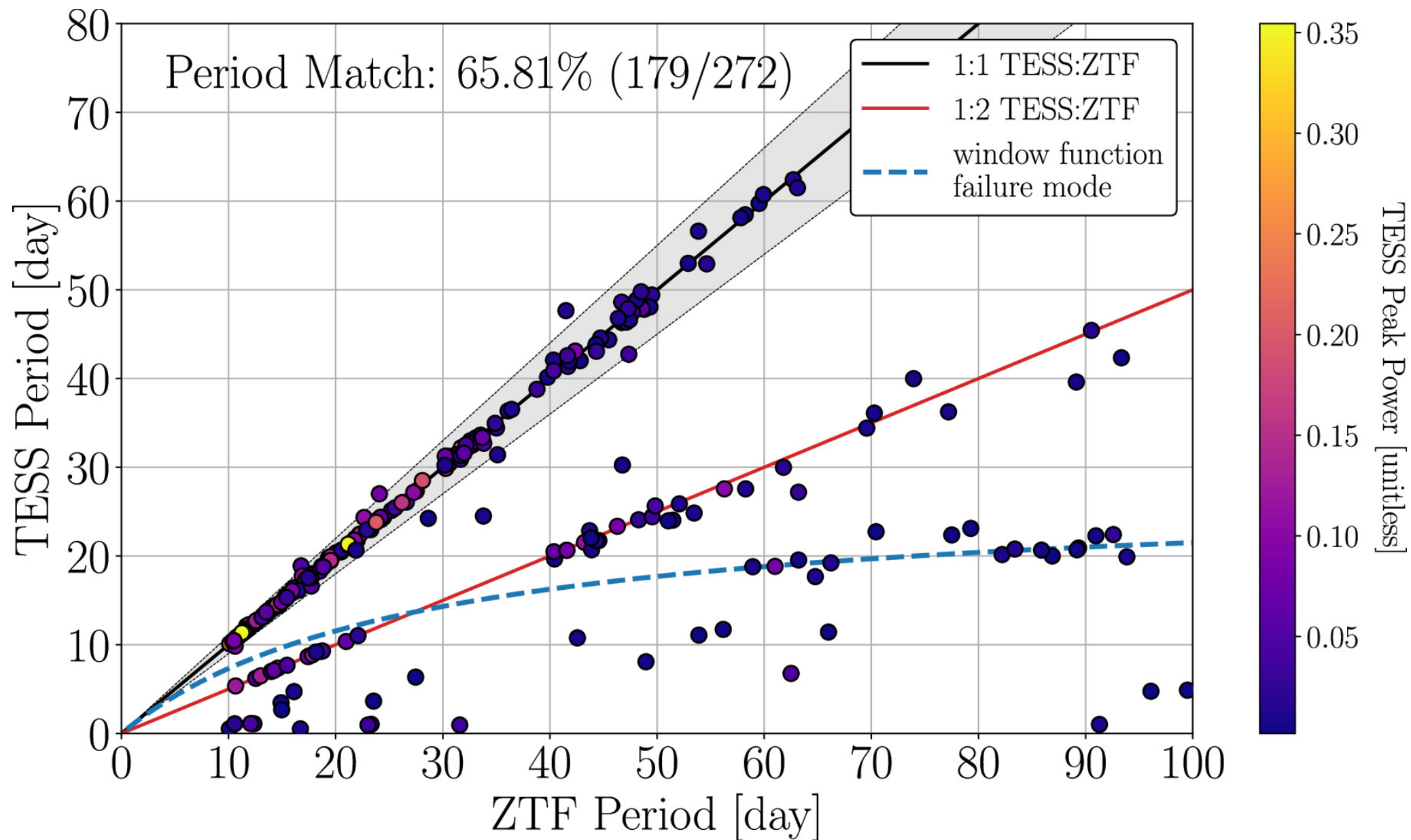
Figure 6. from Soichiro Hattori et al 2025 Astron. J. 170 doi:10.3847/1538-3881/add0ab https://dx.doi.org/10.3847/1538-3881/add0ab © 2025. The Author(s). Published by the American Astronomical Society.
