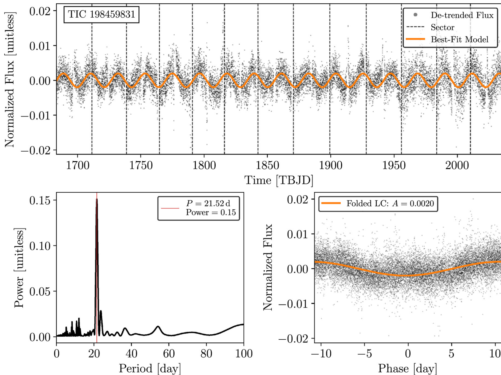
Figure 5. from Soichiro Hattori et al 2025 Astron. J. 170 doi:10.3847/1538-3881/add0ab https://dx.doi.org/10.3847/1538-3881/add0ab © 2025. The Author(s). Published by the American Astronomical Society.
