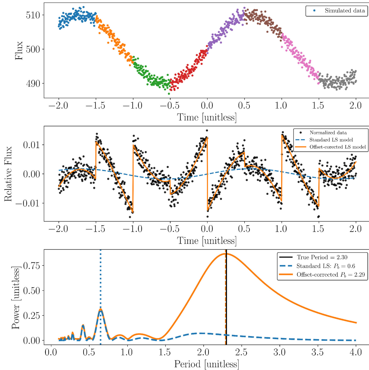
Figure 4. from Soichiro Hattori et al 2025 Astron. J. 170 doi:10.3847/1538-3881/add0ab https://dx.doi.org/10.3847/1538-3881/add0ab © 2025. The Author(s). Published by the American Astronomical Society.
