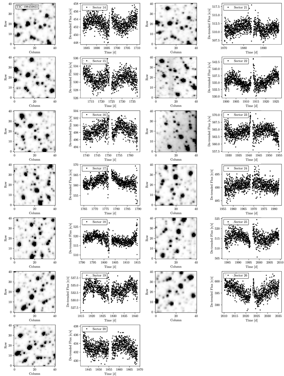
Figure 3. from Soichiro Hattori et al 2025 Astron. J. 170 doi:10.3847/1538-3881/add0ab https://dx.doi.org/10.3847/1538-3881/add0ab © 2025. The Author(s). Published by the American Astronomical Society.
