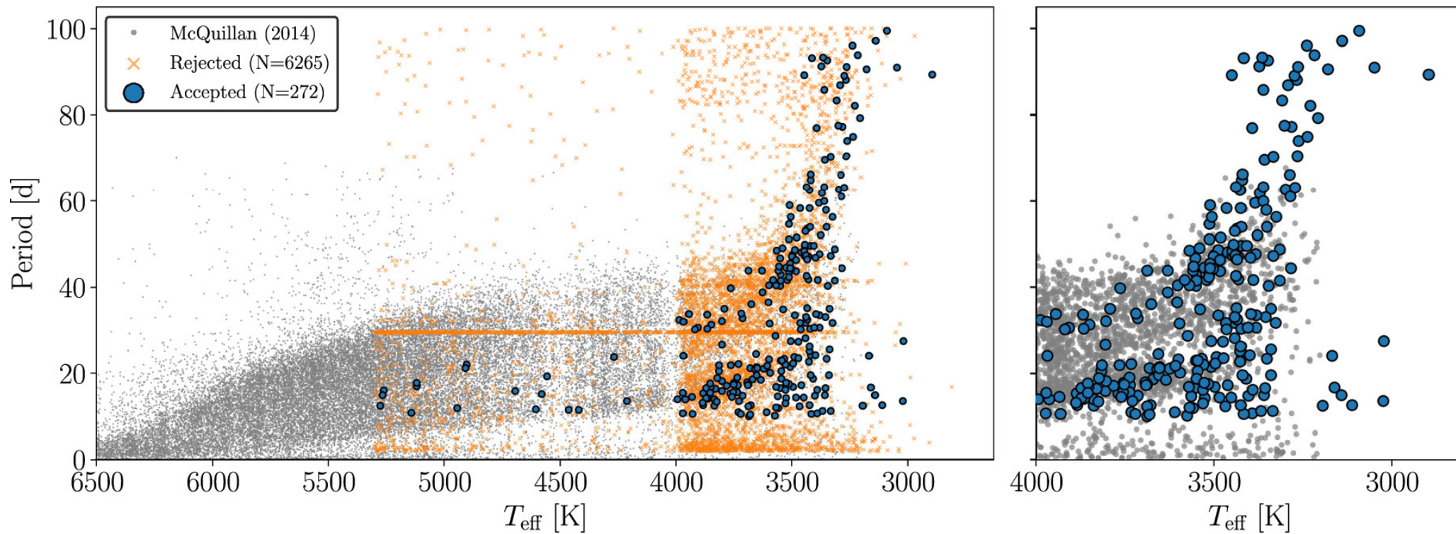
Figure 2. from Soichiro Hattori et al 2025 Astron. J. 170 doi:10.3847/1538-3881/add0ab https://dx.doi.org/10.3847/1538-3881/add0ab © 2025. The Author(s). Published by the American Astronomical Society.
