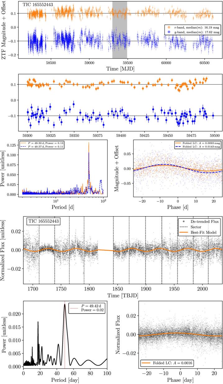
Figure 11. from Soichiro Hattori et al 2025 Astron. J. 170 doi:10.3847/1538-3881/add0ab https://dx.doi.org/10.3847/1538-3881/add0ab © 2025. The Author(s). Published by the American Astronomical Society.
