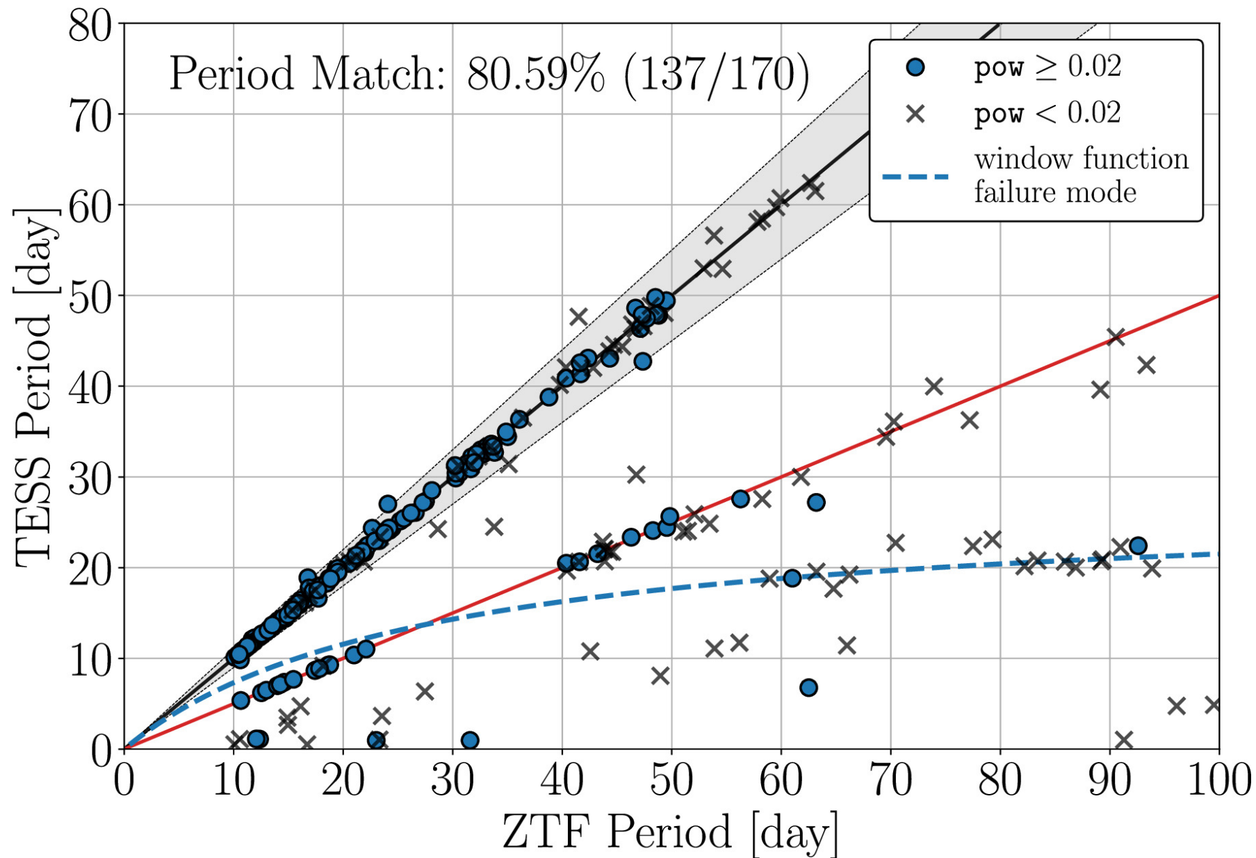
Figure 10. from Soichiro Hattori et al 2025 Astron. J. 170 doi:10.3847/1538-3881/add0ab https://dx.doi.org/10.3847/1538-3881/add0ab © 2025. The Author(s). Published by the American Astronomical Society.
