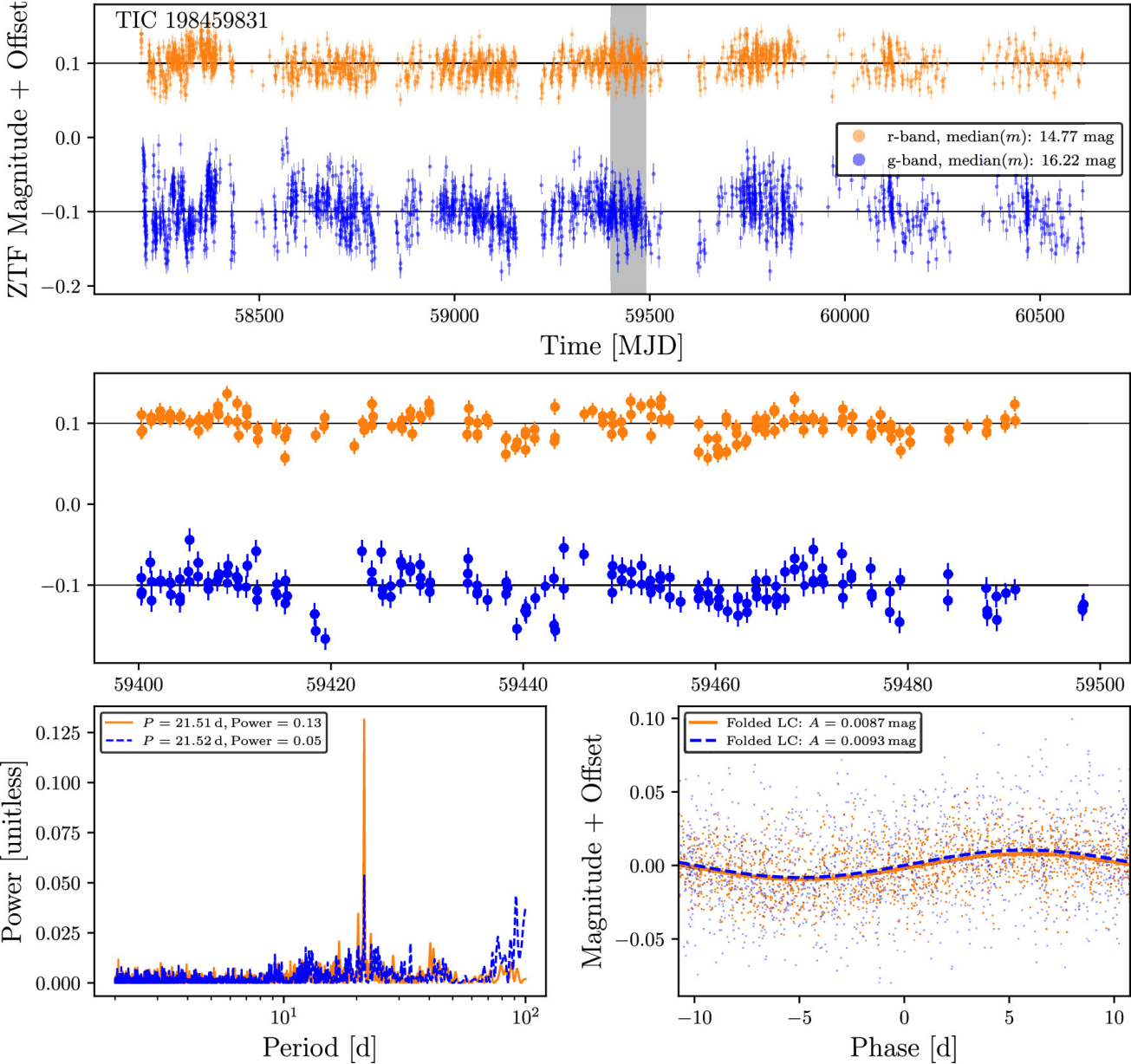
Figure 1. from Soichiro Hattori et al 2025 Astron. J. 170 doi:10.3847/1538-3881/add0ab https://dx.doi.org/10.3847/1538-3881/add0ab © 2025. The Author(s). Published by the American Astronomical Society.
