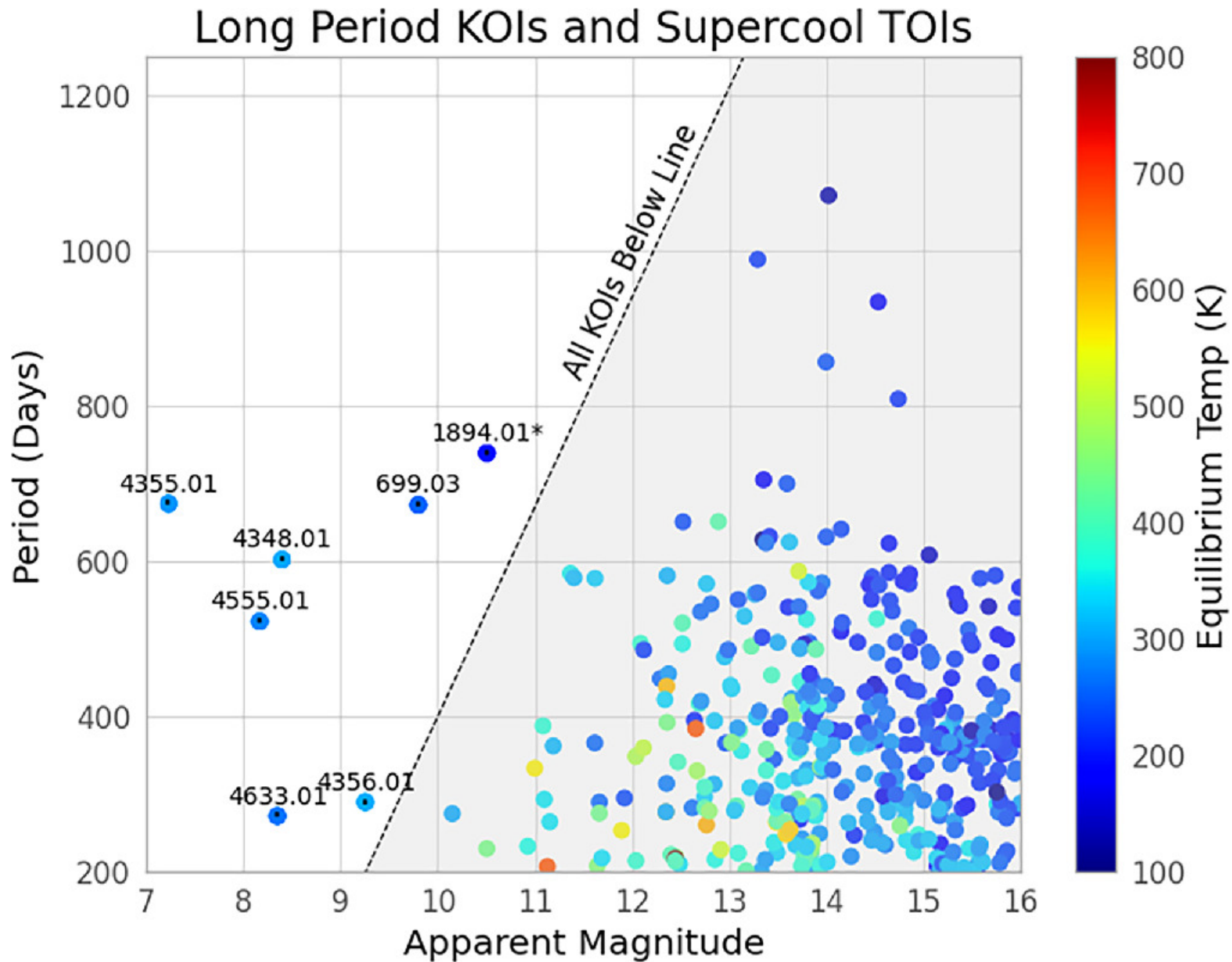
Figure 3. from Dillon J. Bass and Daniel C. Fabrycky 2025 Astron. J. 169 doi:10.3847/1538-3881/adcac6 https://dx.doi.org/10.3847/1538-3881/adcac6 © 2025. The Author(s). Published by the American Astronomical Society.
