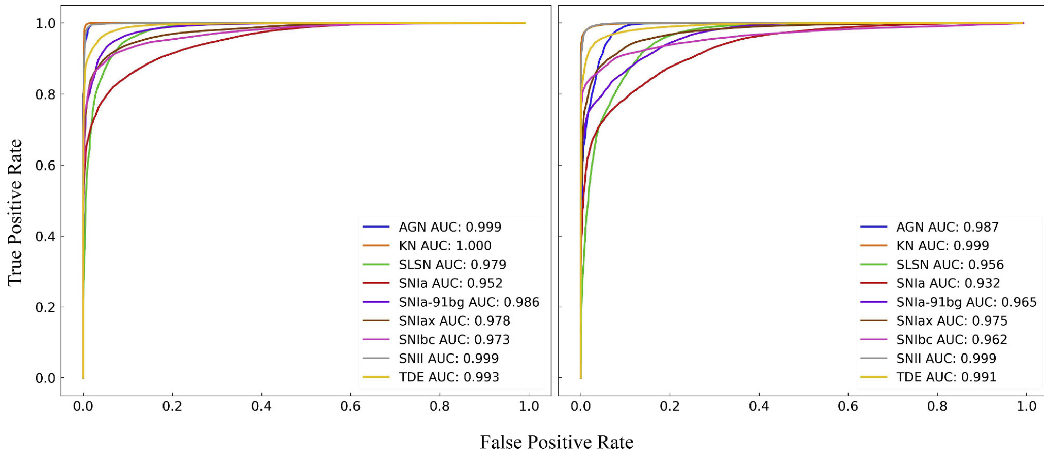
Figure 9. from Yongling Tang et al 2025 Astron. J. 169 doi:10.3847/1538-3881/adcac0 https://dx.doi.org/10.3847/1538-3881/adcac0 © 2025. The Author(s). Published by the American Astronomical Society.
