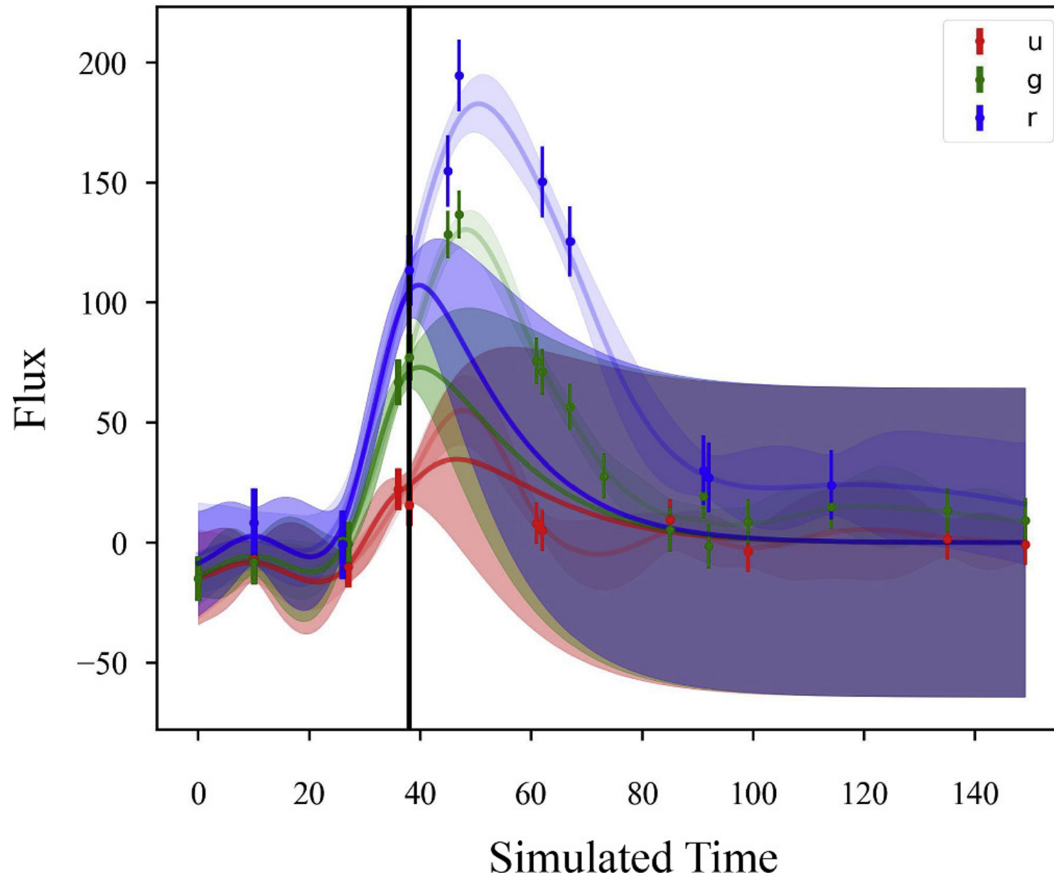
Figure 4. from Yongling Tang et al 2025 Astron. J. 169 doi:10.3847/1538-3881/adcac0 https://dx.doi.org/10.3847/1538-3881/adcac0 © 2025. The Author(s). Published by the American Astronomical Society.
