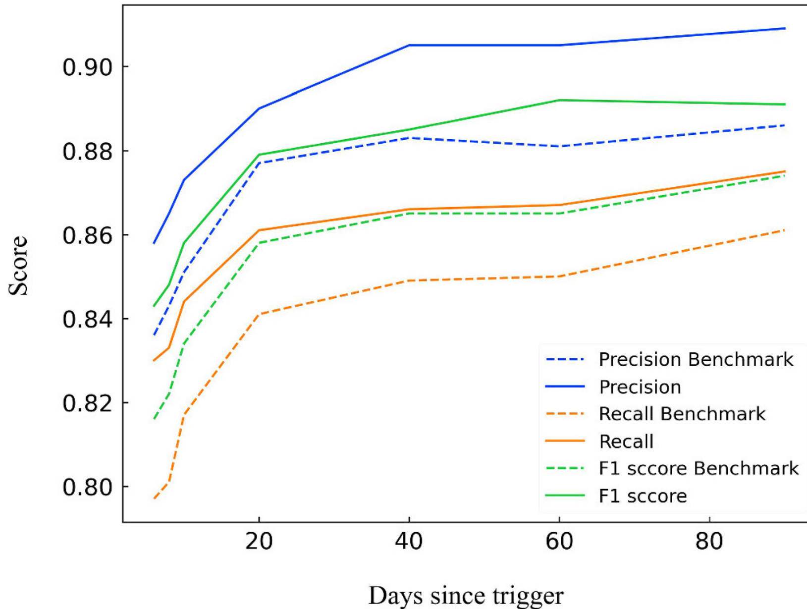
Figure 10. from Yongling Tang et al 2025 Astron. J. 169 doi:10.3847/1538-3881/adcac0 https://dx.doi.org/10.3847/1538-3881/adcac0 © 2025. The Author(s). Published by the American Astronomical Society.
