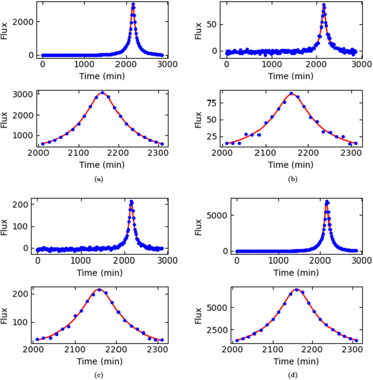
Figure 6. from Michael D. Albrow 2025 Astron. J. 169 doi:10.3847/1538-3881/adc9a1 https://dx.doi.org/10.3847/1538-3881/adc9a1 © 2025. The Author(s). Published by the American Astronomical Society.
